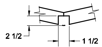
KEELSON CUTOUT TYPICAL ALL FRAMES
