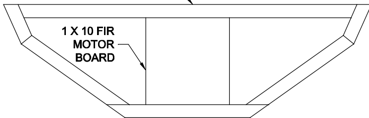
TRANSOM FRAMING & FAIRING DETAIL SCALE = 1/5
