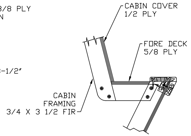
FORWARD SECTIONS CABIN CONSTRUCTION NO SCALE
