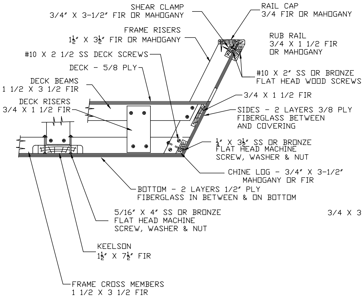
CONSTRUCTION DETAIL TYPICAL AT AFT SECTION NO SCALE
