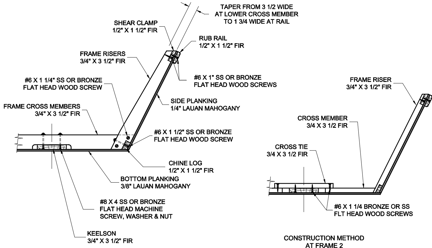
CONSTRUCTION METHOD TYPICAL AT FRAMES 1 & 3
