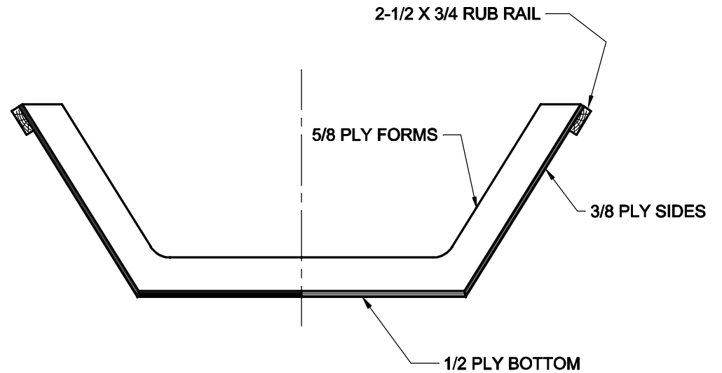
CROSS SECTION AFT
