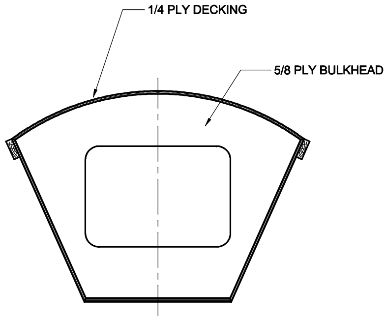
CROSS SECTION FORWARD
