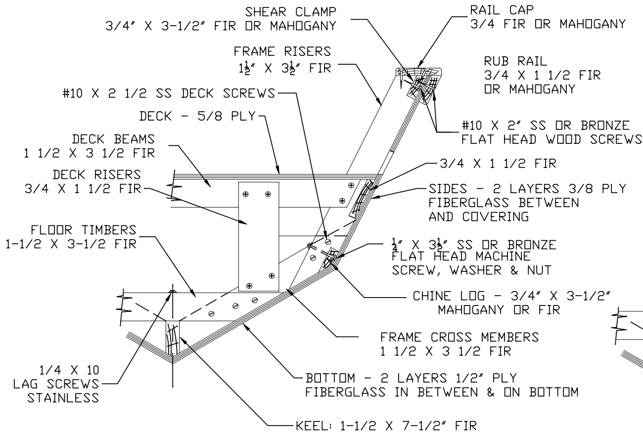
CONSTRUCTION DETAIL TYPICAL AT AFT SECTION NO SCALE
