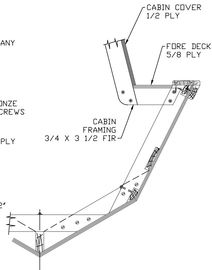
FORWARD SECTIONS CABIN CONSTRUCTION NO SCALE
