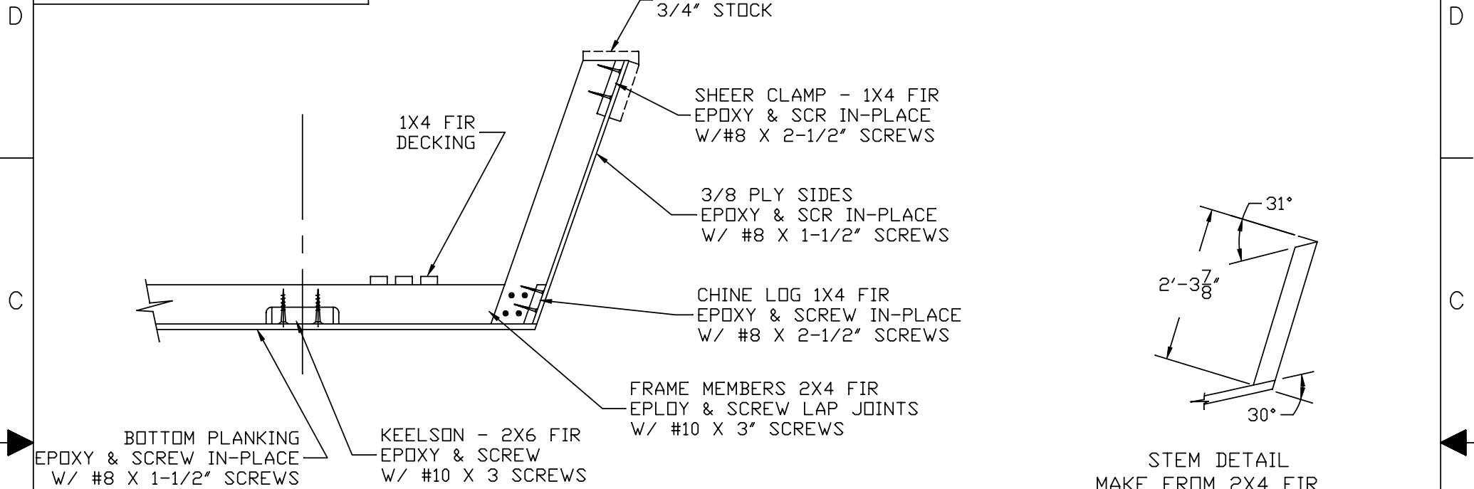
TYPICAL CONSTRUCTION METHOD ALL FRAME STATIONS SCALE 2" = 1'
