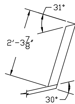
STEM DETAIL MAKE FROM 2X4 FIR
