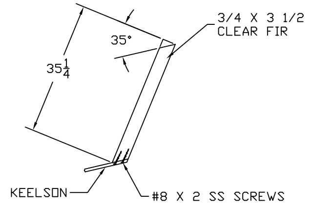
STEM DETAILS
