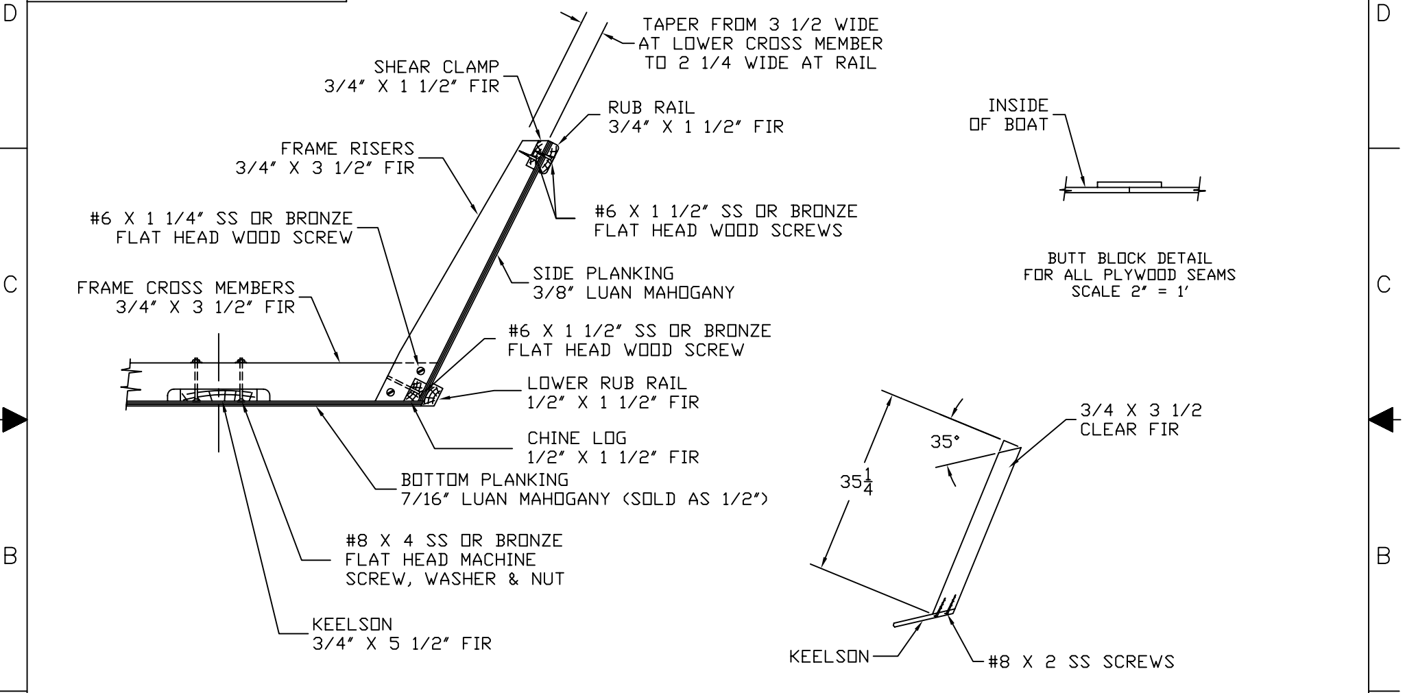
STEM DETAILS
